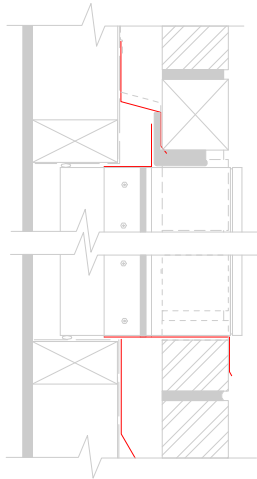
Cross section
