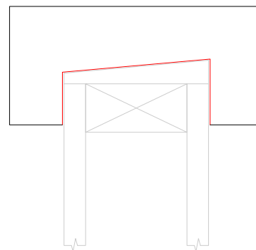
Saddle flashing over framing
